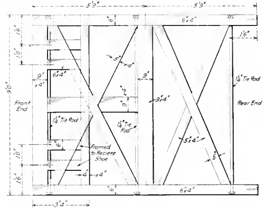
Snow Plow Frame
